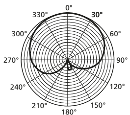
9 Diagrama polar vertical
