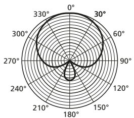
8 Diagrama polar horizontal
